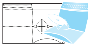
CD Pop Up Mailer 1-up 8.625 x 4.9375 pre taped
