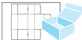
General Purpose Box 1-up 4.75 x 3.1 x 2
