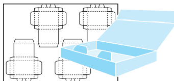
Playing Card Box 4-up 2.5 x 3.625 x .75
