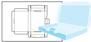
Photo Card Box 4 x 6 1-up 4.5 x 6.5 x .75
