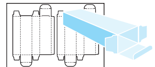
Toothpaste Box 2-up 2.125 x 7.125 x 1.375
