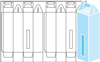
Wine Bottle Box 2-up 3.23 x 3.23 x 13.125
