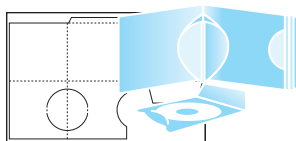
DVD Pop Up Mailer 1-up 5.25 x 5.25 x .125
