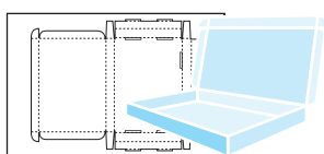
Greeting Card Box 1-up 5.5 x 7.75 x .75
