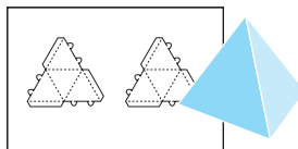
Pyramid Box 2-up 3 x 3 x 3
